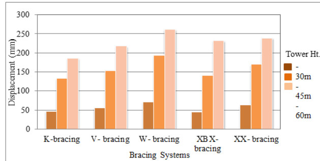
Fig 3: Variation of Displacement (mm) at Top for Different Tower for Zone-VI
