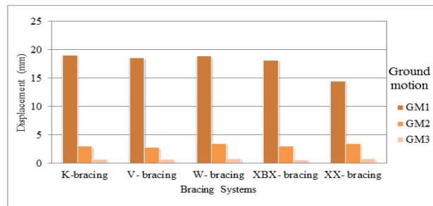
Fig 5: Variation of Displacement (mm) at Top with 45m tower Different Bracing for ground motions in x-direction
