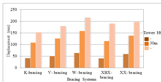
Fig 2: Variation of Displacement (mm) at Top for Different Tower for Zone-V
